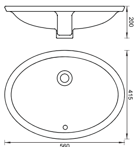
Big UNDER COUNTER BASIN CAT NO. SP7029 560 X 415 X 200 MM
